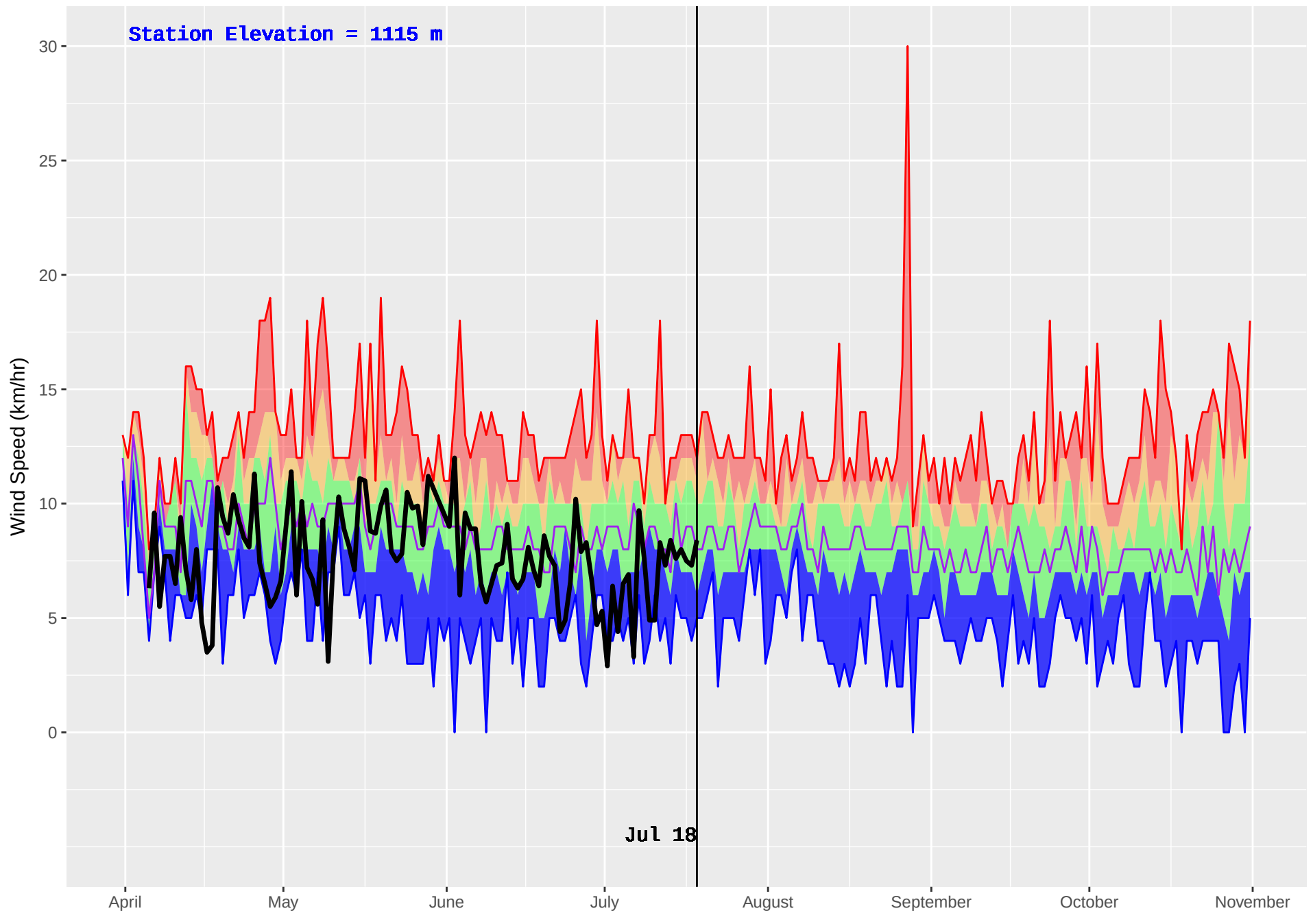
SICAMOUS (882) : Historical (2004–2016) and Current (2018) Daily Wind Speed
