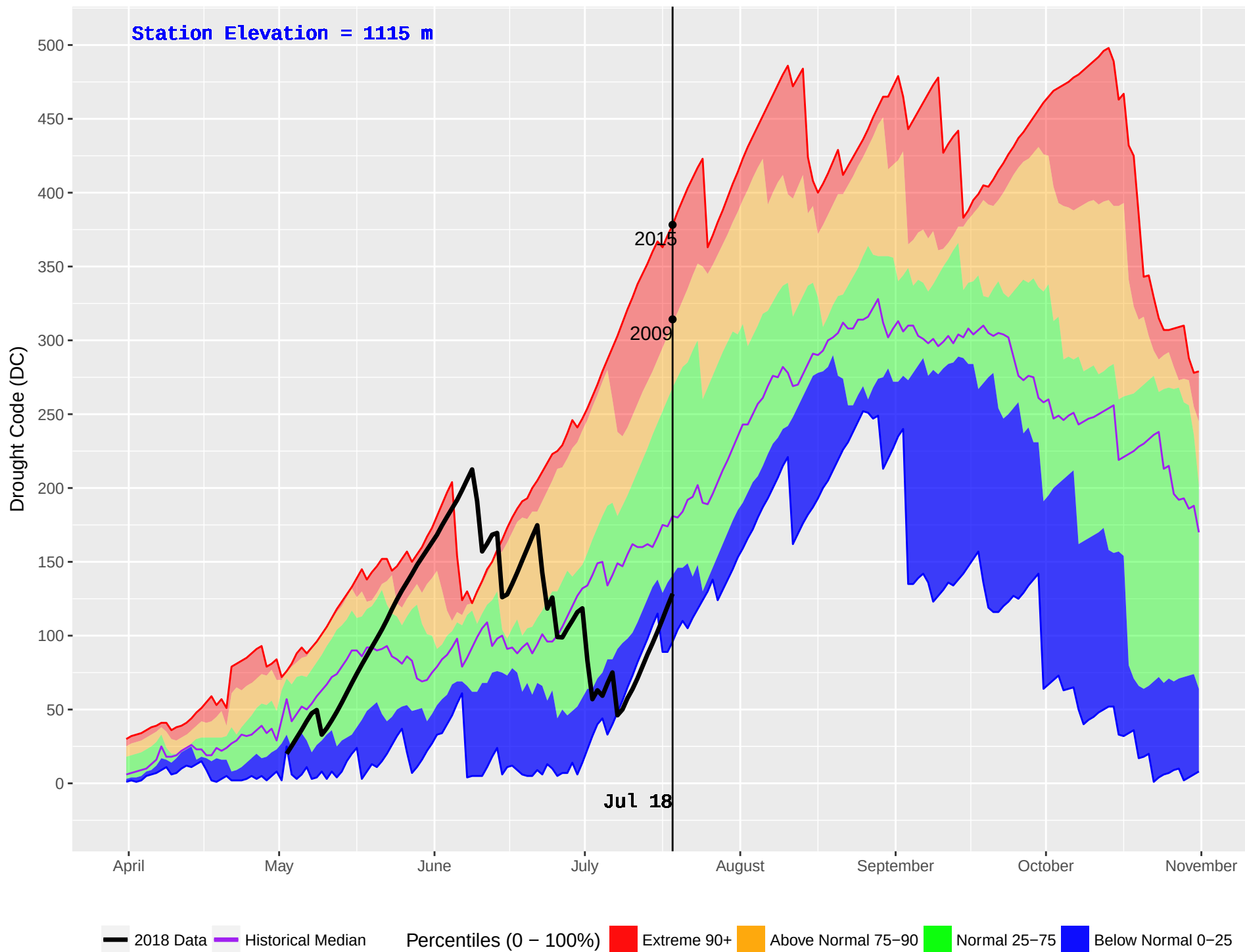
SICAMOUS (882) : Historical (2004–2016) and Current (2018) Daily Drought Code (DC)
