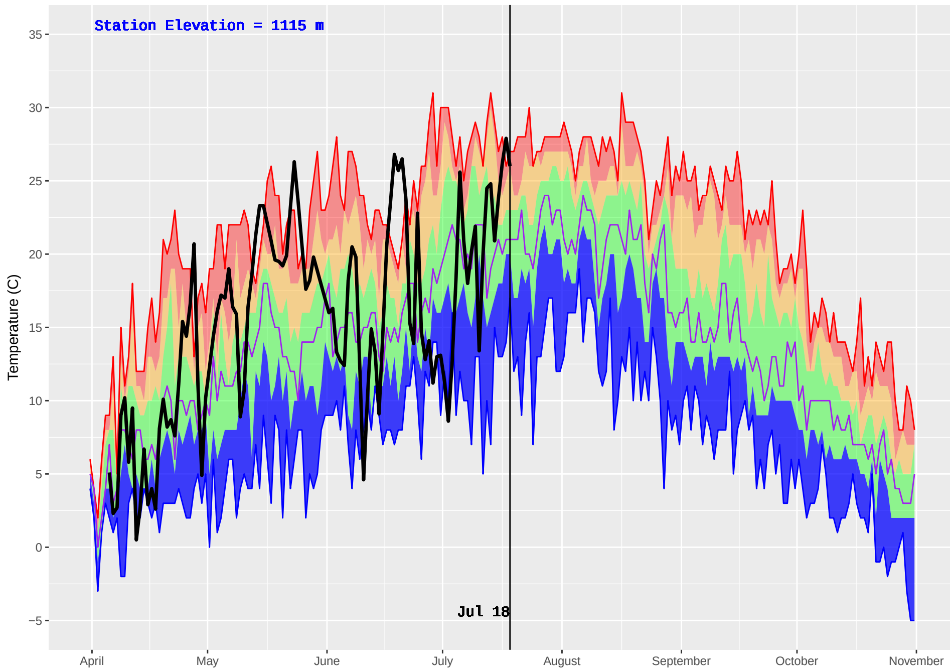
SICAMOUS (882) : Historical (2004–2016) and Current (2018) Daily Temperature
