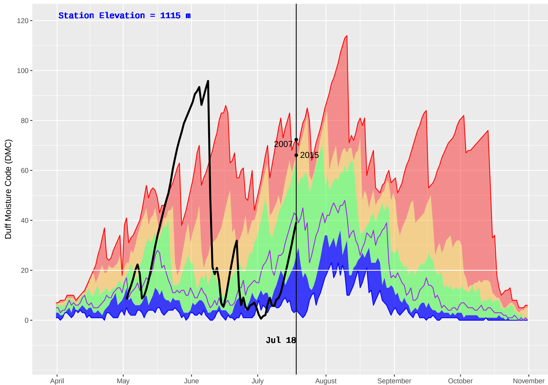
SICAMOUS (882) : Historical (2004–2016) and Current (2018) Daily Duff Moisture Code (DMC)
