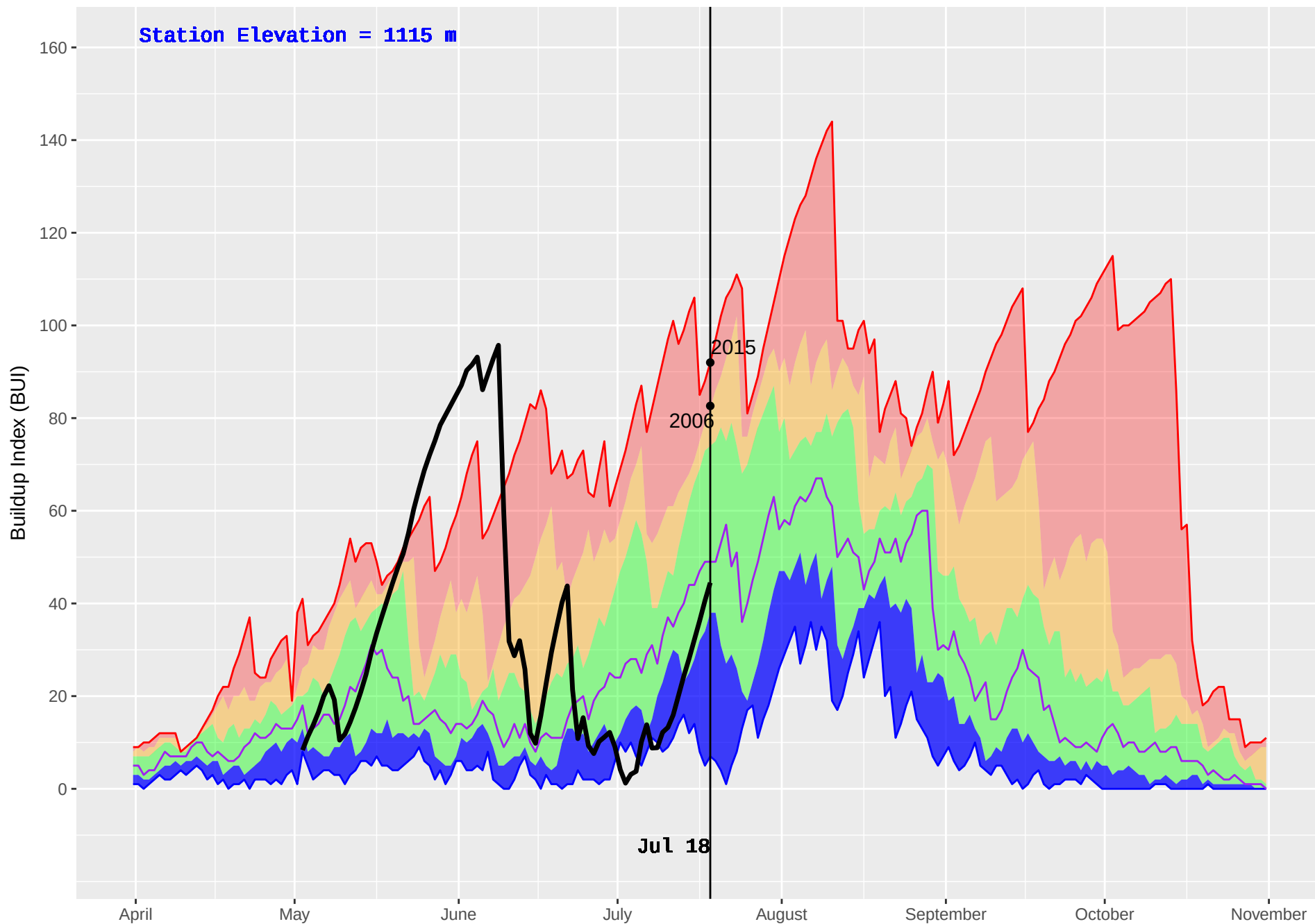
SICAMOUS (882) : Historical (2004–2016) and Current (2018) Daily Buildup Index (BUI)
